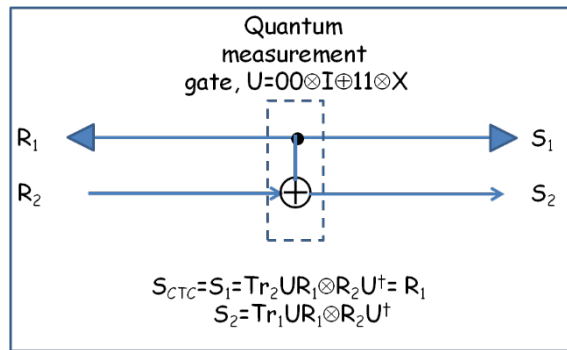
Fig. 9a. CTC circuit with ► representing wormhole input port and ◄ representing wormhole output port.
