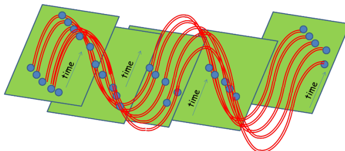
Fig. 12. The Multiverse as perhaps envisioned by David Deutsch connected by CTC wormholes.
